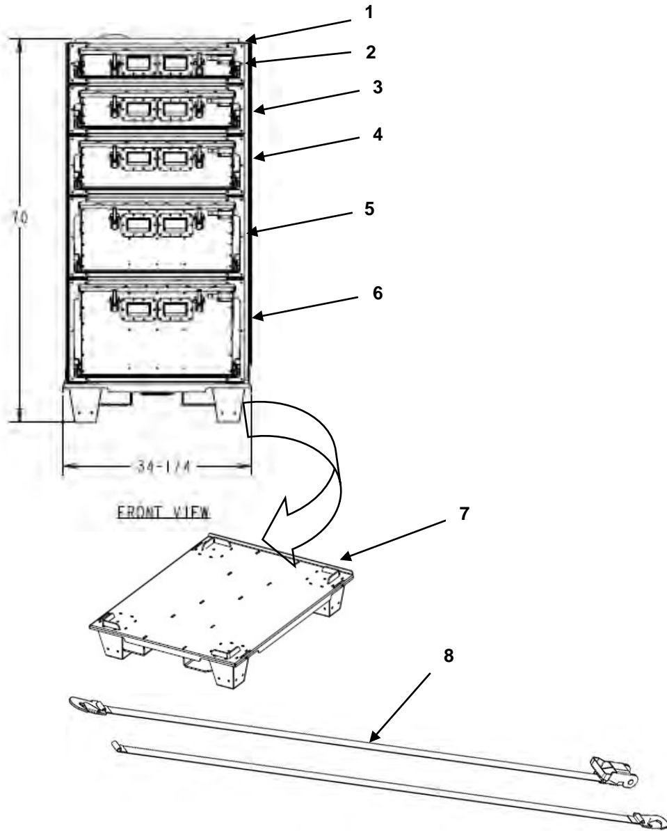
FIGURE 04 PDM CONFIGURATION # 03
