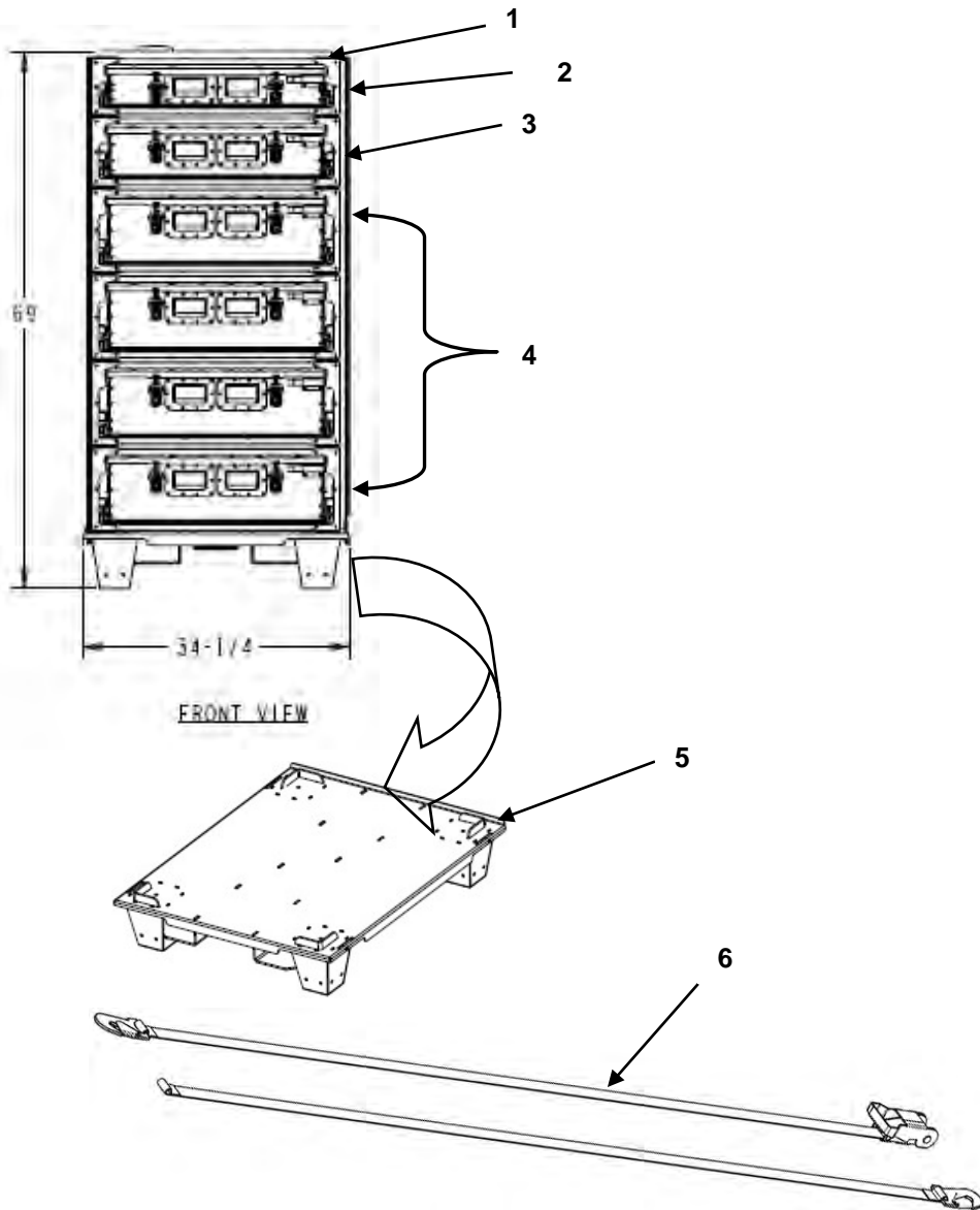
FIGURE 05 PDM CONFIGURATION # 04
