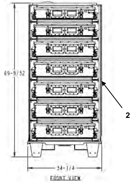
PDM CONFIGURATION #4
